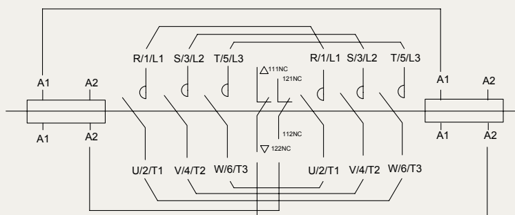
<MC-6aR(Q) ~ MC-150aR(Q) typical circuit diagram for reversing contactor>
